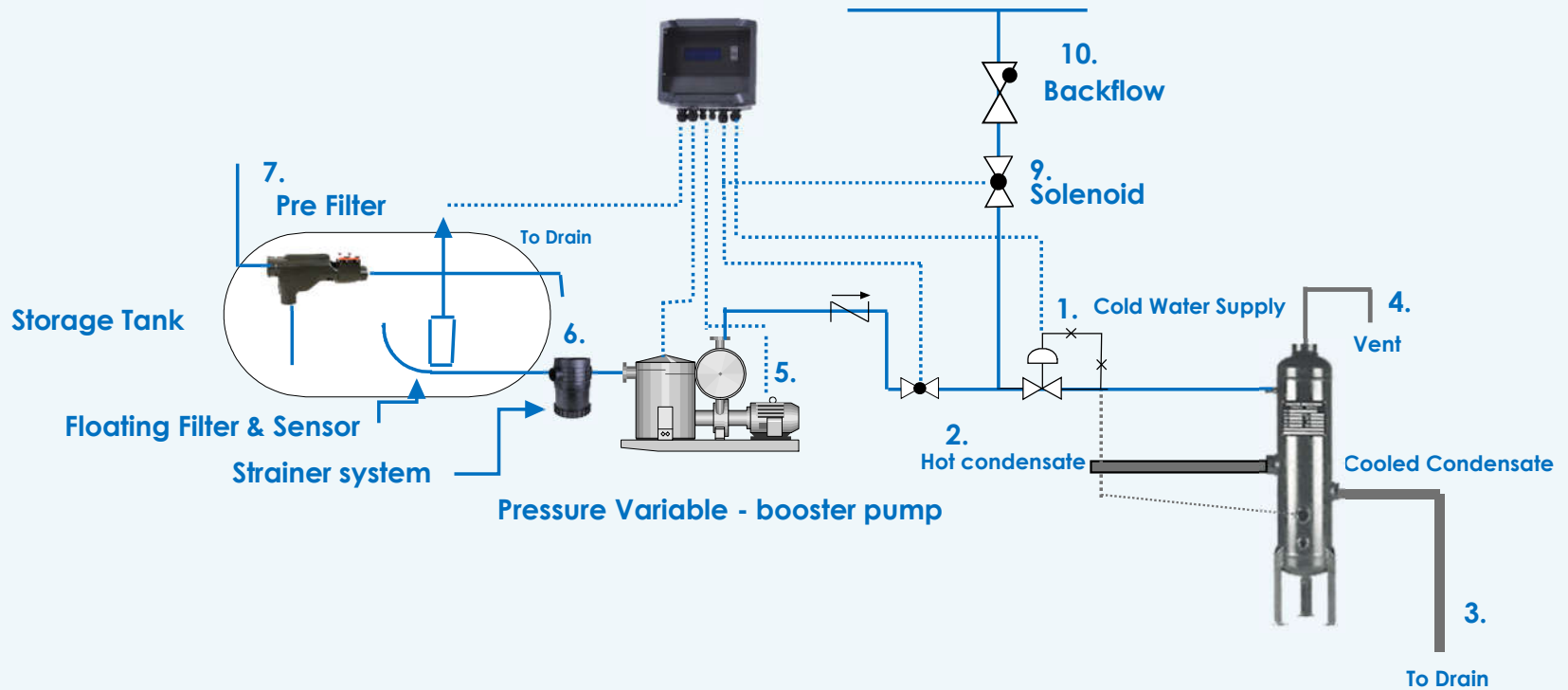
Typical Condensate Cooler
